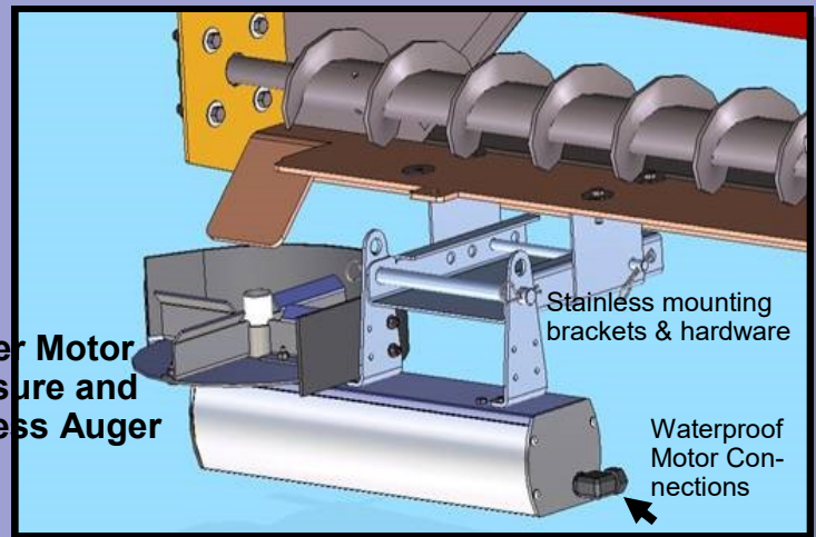
Waterproof Rear Motor Connectors
