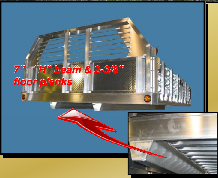
TC501 SHOWN WITH OPTIONAL HEADBOARD, TAILBOARD, DROP-SIDES
